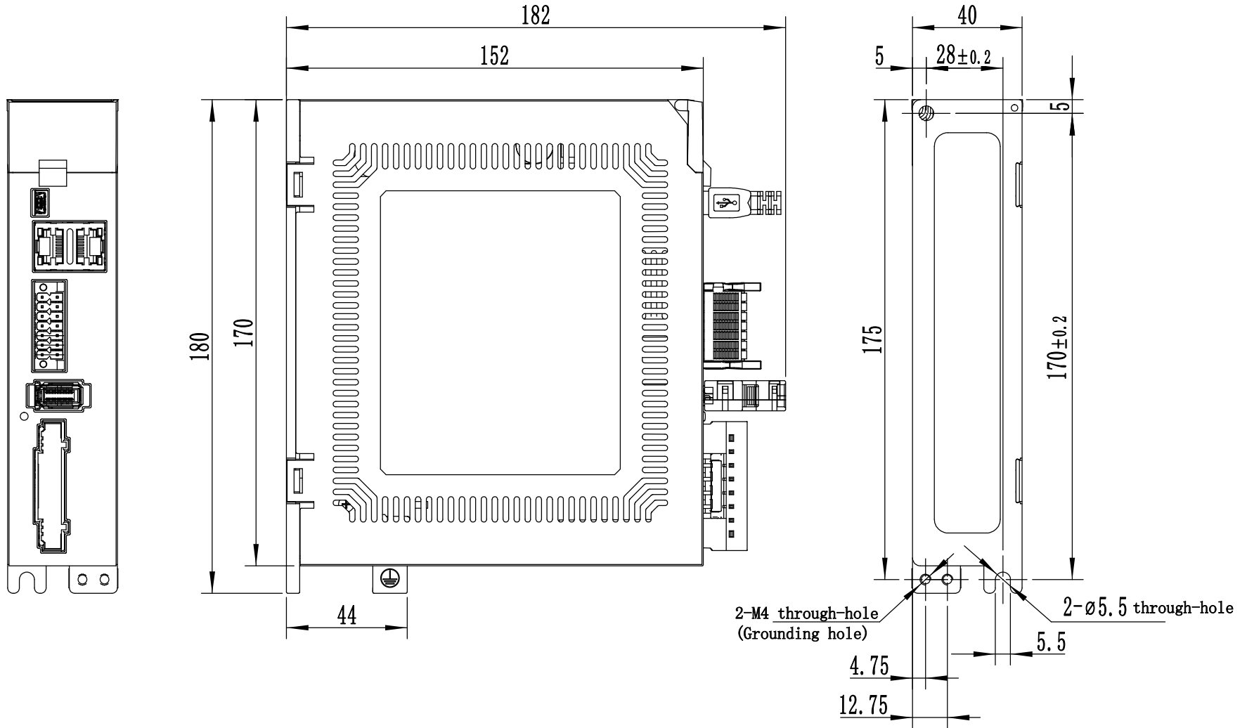
M54S-23A0ECN尺寸图 M54S-23A0ECN 2D drawing
