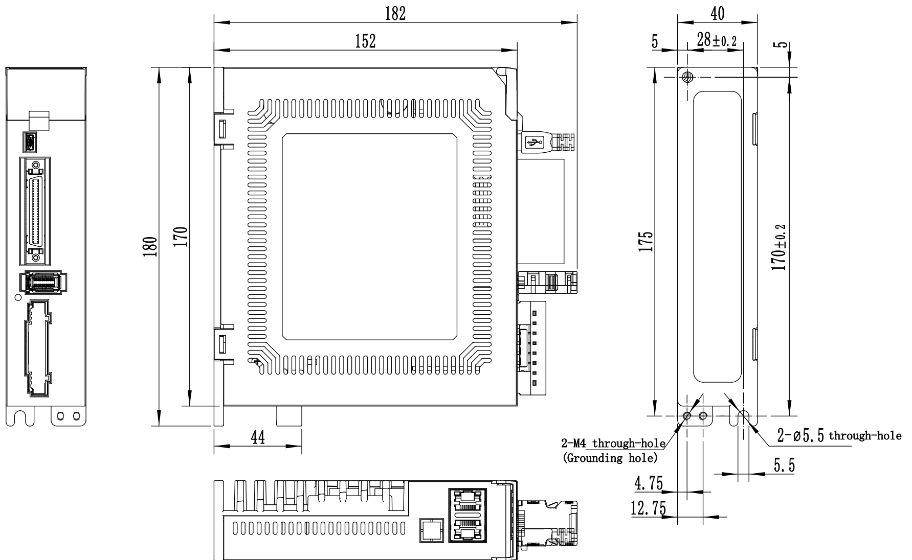
M54S-23A0RD 尺寸图 M54S-23A0RD 2D drawing
