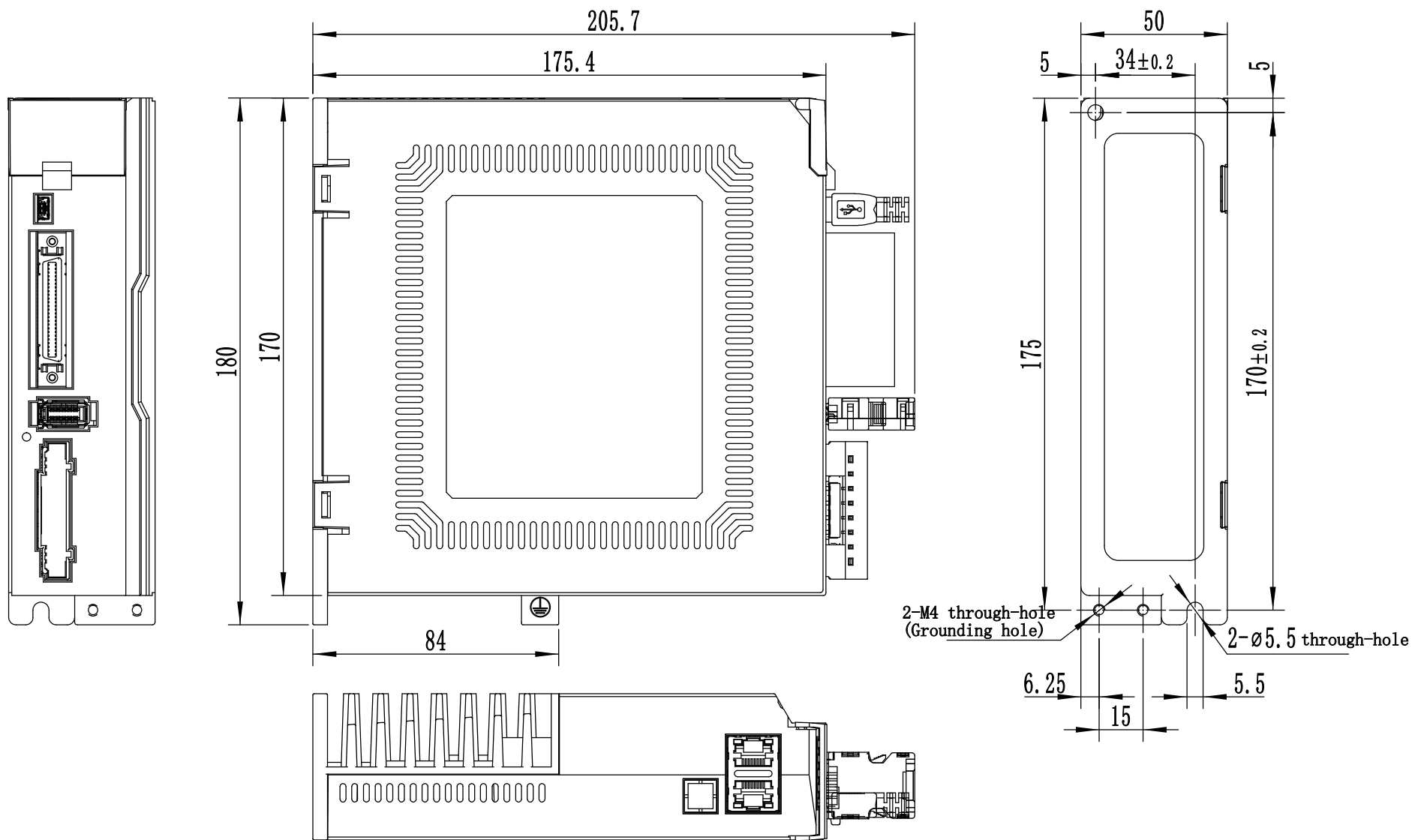
M54S-24A5RD 尺寸图 M54S-24A5RD 2D drawing
